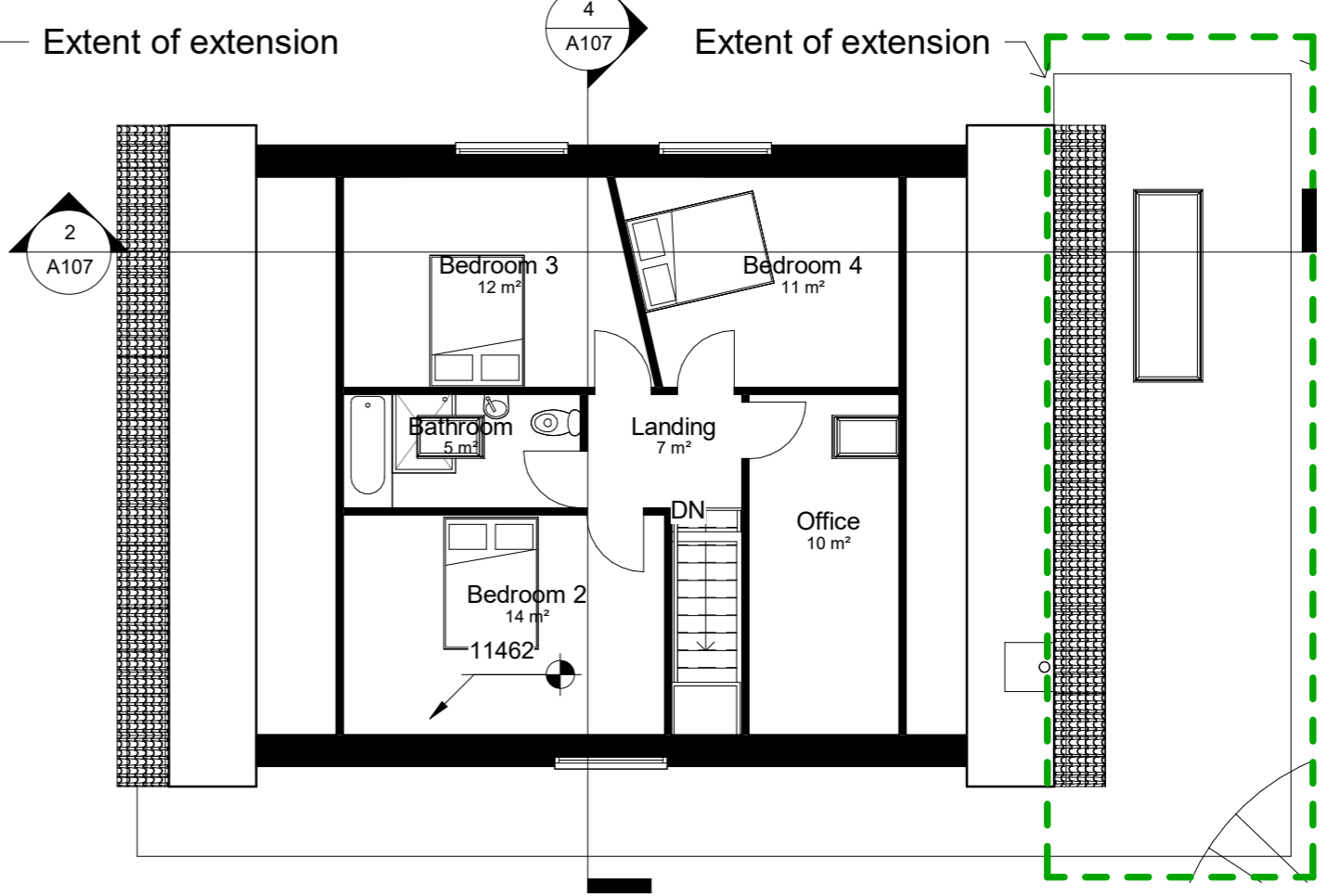
2 Level 1 - Proposed 1 : 100
