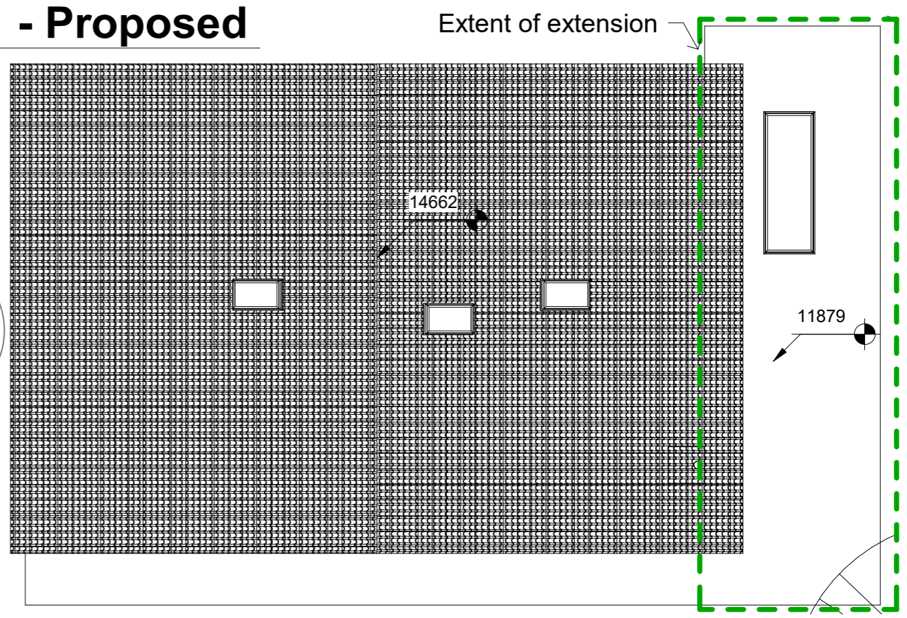
3 Roof - Proposed 1 : 100
