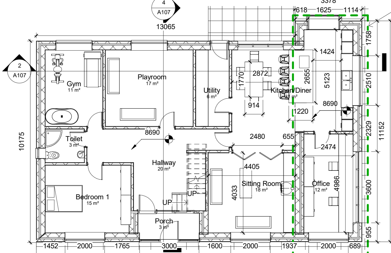
1 Level 0 - Proposed 1 : 100
