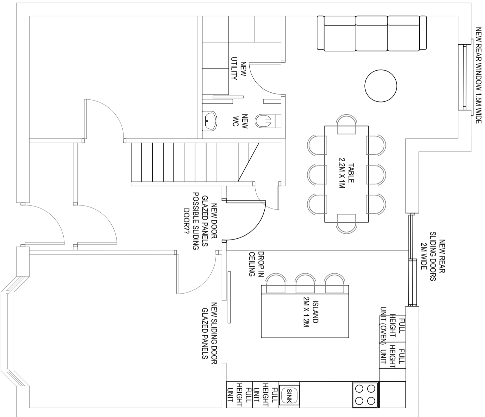
OPTION 1B PROPOSED GROUND FLOOR PLAN (WITHOUT DEMOLITIONS SHOWN) SCALE 1:50 @ A3
