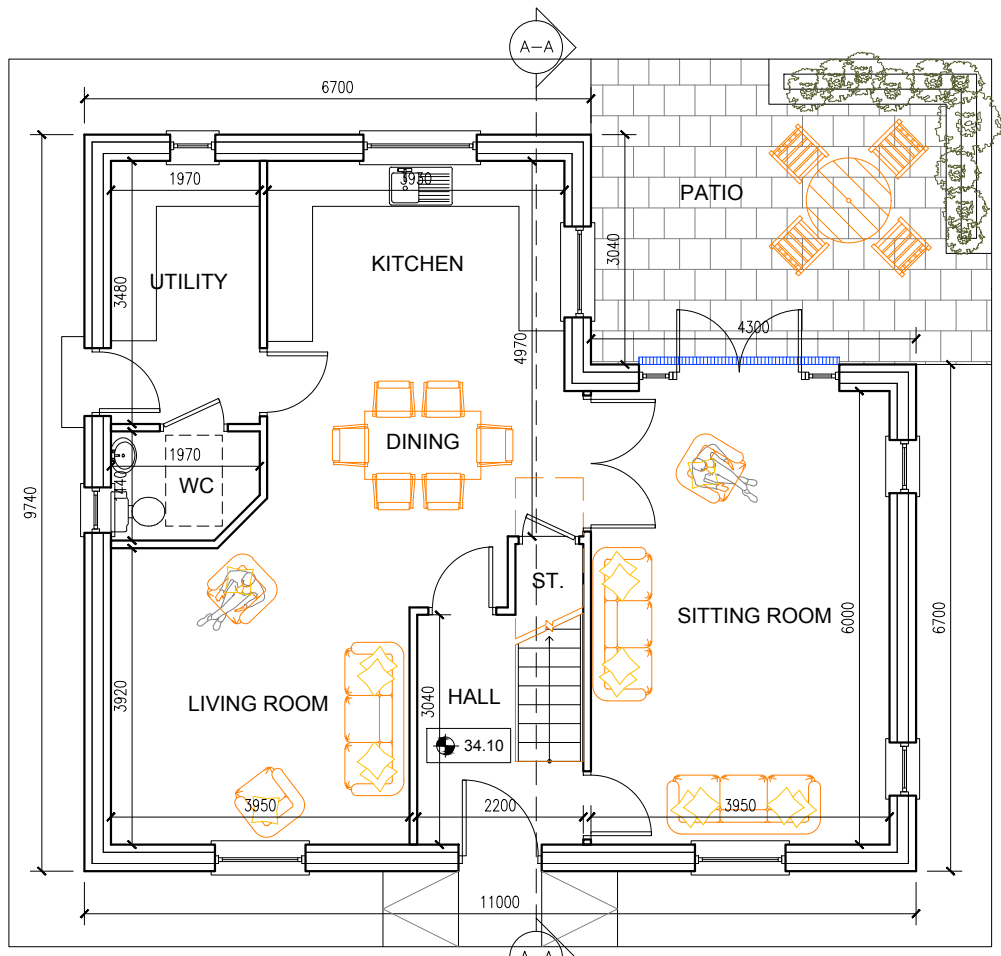
GROUND FLOOR PLAN (Floor Area = 80m 2 / 861ft 2 )
