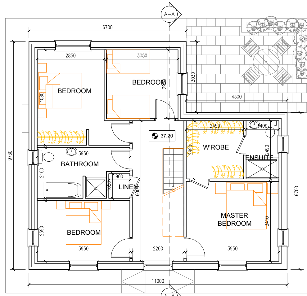
FIRST FLOOR PLAN (Floor Area = 80m 2 / 861ft 2 )
