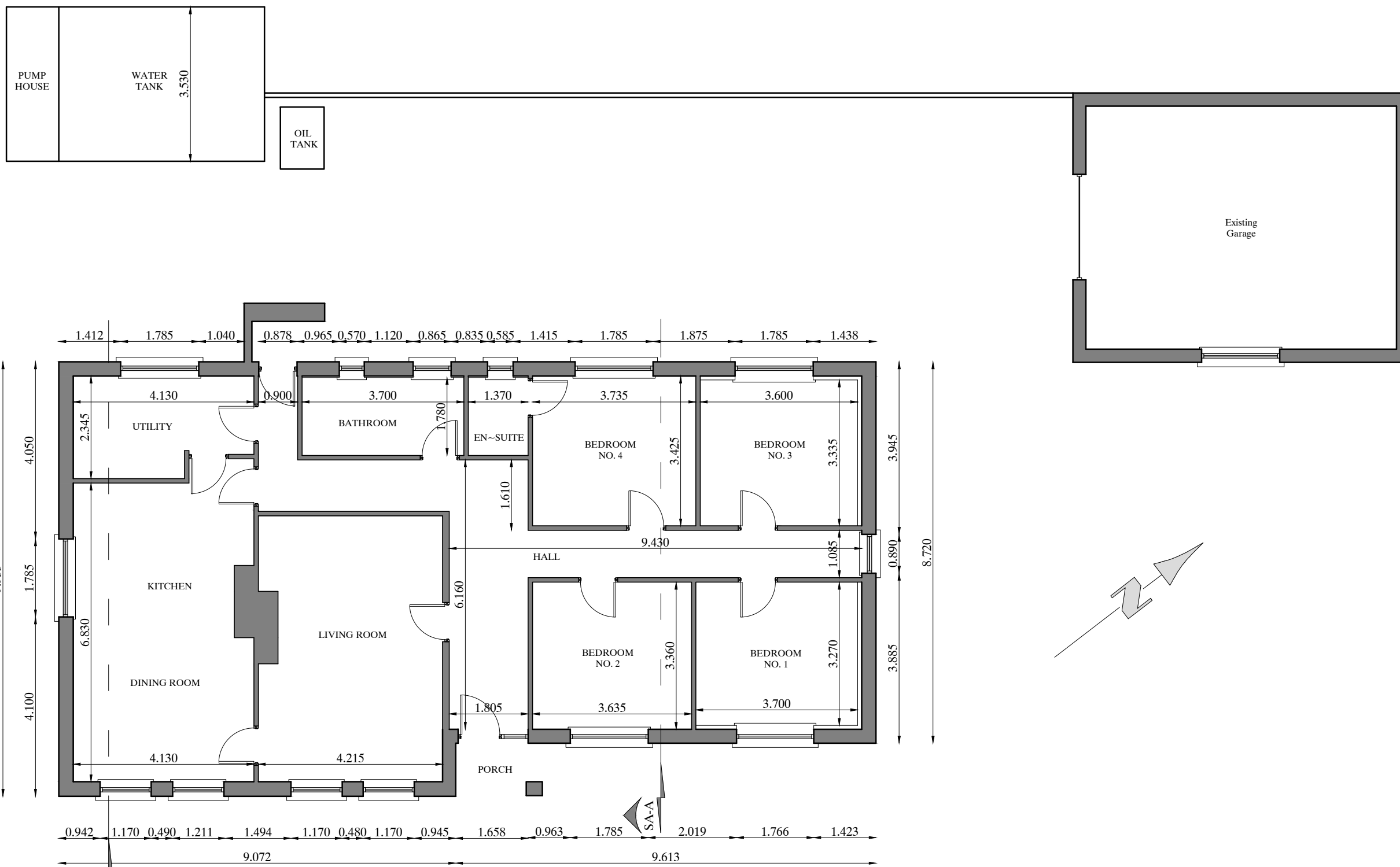
G EXISTING GROUND FLOOR PLAN Total Ground Floor Area = 156 m 2 (1,679 ft 2 ) ~ Scale 1:100
